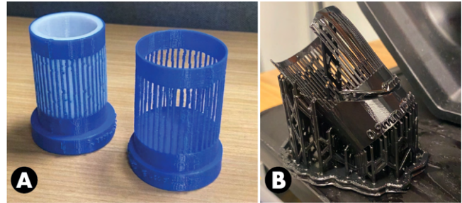
Figure 9: (A) The FDM sample shows inconsistent fringe spacing and also warping. (B) The SLA object has support structures bonded to the Moiré fringes which are difficult to remove and cause significant warping and distortions.
