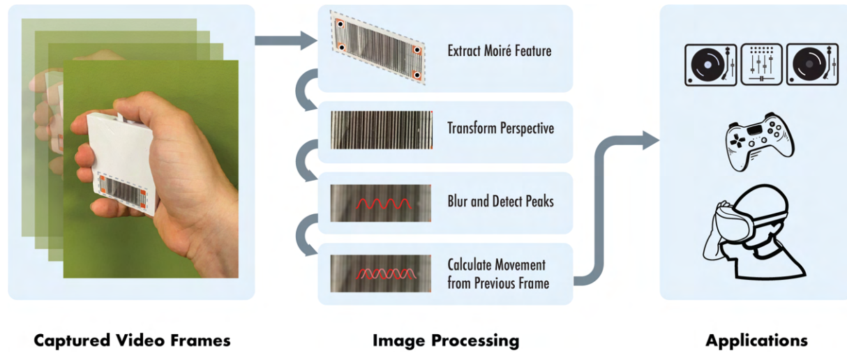
Figure 5: Our image processing pipeline takes captured video frames and extract the Moiré feature with the color markers at the corners. It crops out the rest of the image and applies a perspective transform. We then blur the Moiré fringes, detect the peaks in the visual signal, and calculate the displacement.
