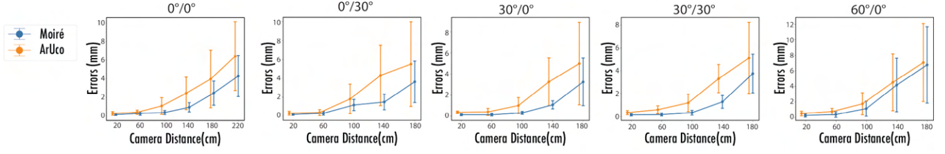
Figure 7: The results of our evaluation. Each plot represents the results at a specific camera angle ( X^\circ/Z^\circ ) with respect to distance changes in cm . The line segments show the RMSE measurement in mm , and the bars indicate the standard deviation of the error. Both our method and ArUco were measured under the same conditions. The ArUco plot is slightly shifted to the left for a clearer comparative visualization.
